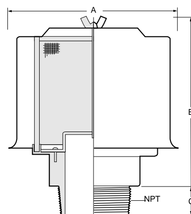
HC-120-T-40P
