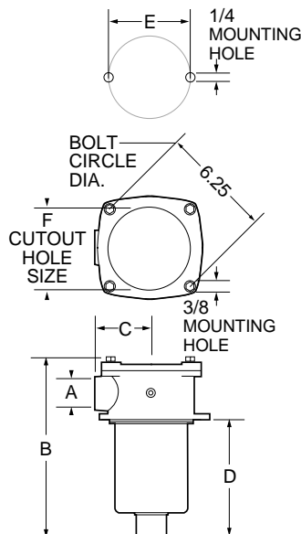
TRFA 08 TRFA 12 TRFA 16 2-HOLE MOUNT
