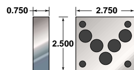
DO5 Cover Plate
