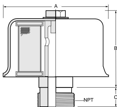
HC-120-T-24P
